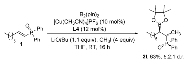
Scheme 3. Methylboration of \alpha,\beta -unsaturated phosphine oxide 1 . Conditions: 1a (0.5 mmol), B_2(\text{pin})_2 (0.75 mmol), THF (1.5 mL). Full conversion; 2i/2a = 71:29 as determined by ^{31}\text{P} NMR spectroscopy and GC analysis.
