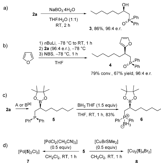
Scheme 4. Stereospecific transformations at the boron and phosphorus functional groups. [a] Conditions A: \text{HSiCl}_3 , \text{Et}_3\text{N} , toluene, 90^\circ\text{C} , 16 h, 66% yield; conditions B: bis(4-nitrophenyl) hydrogen phosphate (7.5 mol%), (\text{EtO})_2\text{MeSiH} (4 equiv), toluene, 110^\circ\text{C} , 16 h, 77% conversion, 58% yield.
